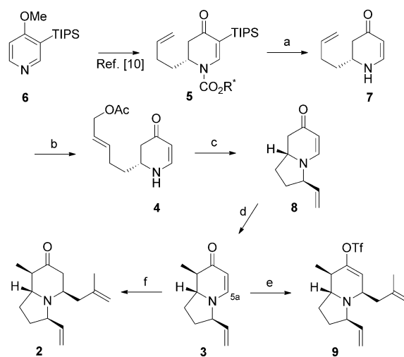
Scheme 2. Synthesis of intermediate 2 . a) MeONa/MeOH, reflux (81 %); b) ( Z )-but-2-ene-1,4-diyl acetate, Grubbs–Hoveyda 2nd-generation cat., CH 2 Cl 2 , reflux (88 %); c) [Pd 2 (dba) 3 ]·CHCl 3 , P( t Bu) 3 , Cs 2 CO 3 , 1,4-dioxane, 75 °C (80 %); d) LDA, THF, –78 °C; MeI, –78 to 0 °C; LDA, –78 °C (82 %, one pot); e) methallyltributylstannane, Tf 2 O, CH 2 Cl 2 , –78 °C (65 %); f) methallyltributylstannane, TFAA, CH 2 Cl 2 , –50 to 0 °C (69 %). dba = dibenzylideneacetone, LDA = lithium diisopropylamide, Tf = trifluoromethanesulfonyl, TFAA = trifluoroacetic anhydride, THF = tetrahydrofuran.
